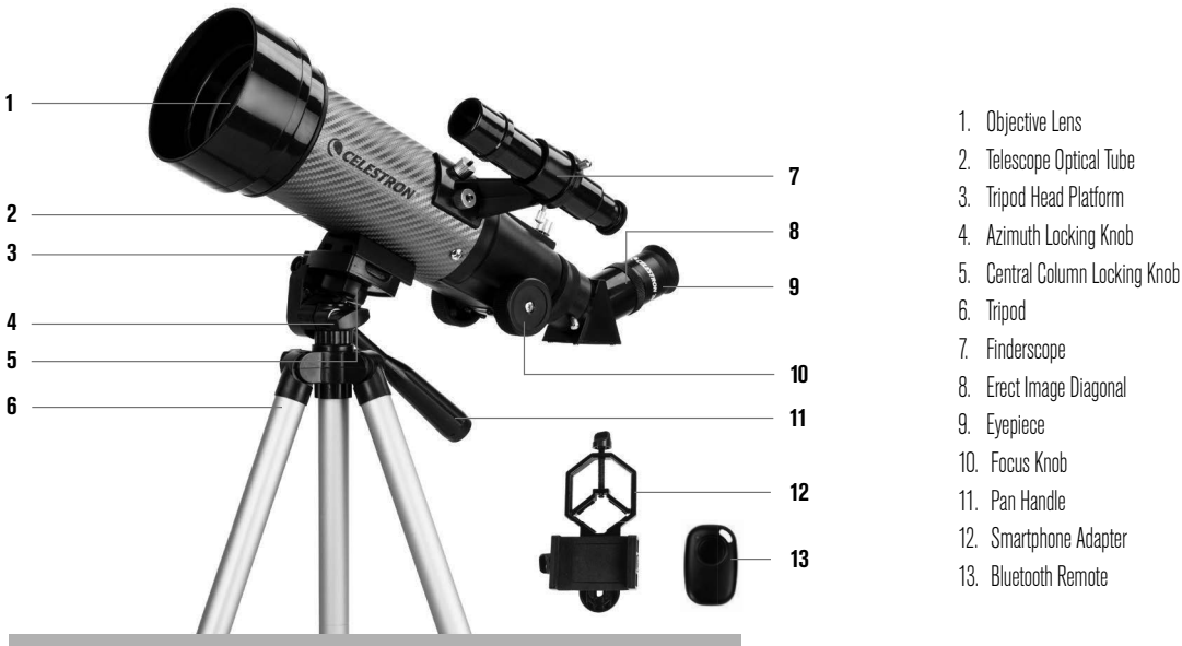
Fig. 1 Travel Scope 70DX (Similar to Travel Scope 60DX)
