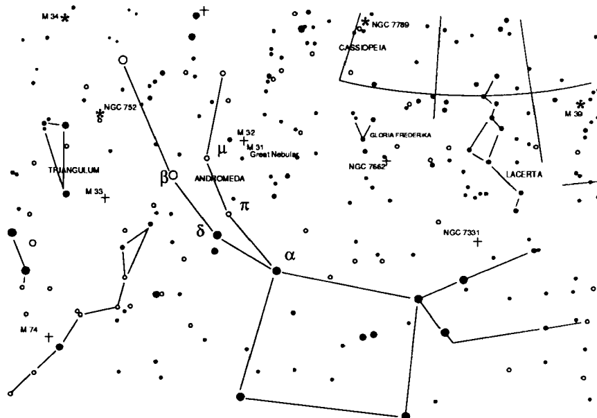
Fig. 16 Galassia Andromeda
